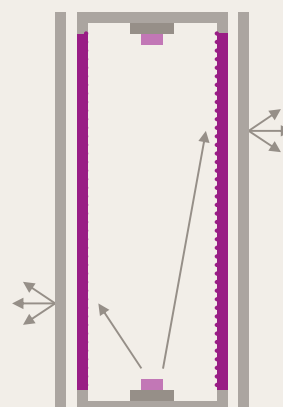
Fig. 2: Cross-section of unit with WH46 SC installed as a diffuser sheet with a backlit poster
