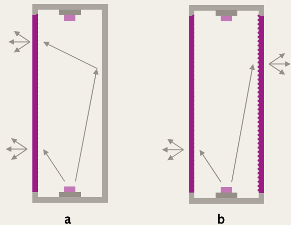
Fig. 1: Cross-section of side-lit light box with WH46 SC installed as a mirror, and LED modules at the top and bottom. (a) one luminous side, (b) two luminous sides
